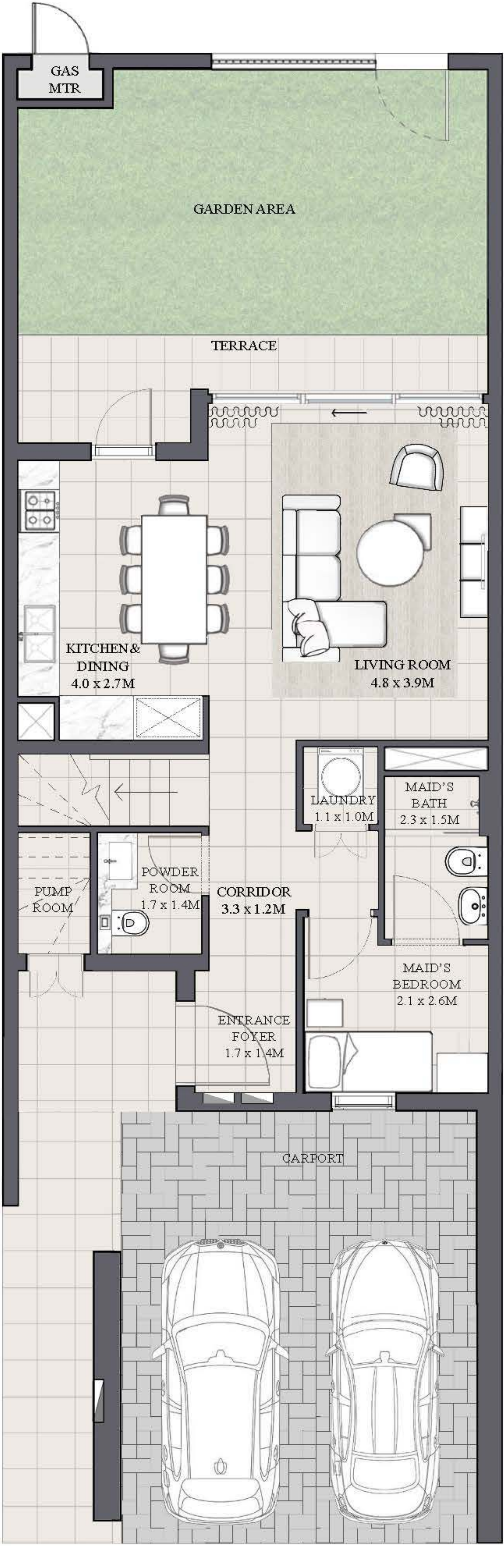
GROUND FLOOR
